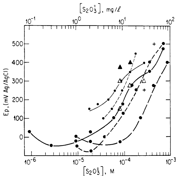
FIGURE 1 — Variations of the pitting potential in 7.0 \times 10^{-4} M \text{Cl}^- solutions at (a) 24 C for Alloy 600 (● — ●); Alloy 800 (○ — ○); AISI 304 SS (Δ, ▲, + for repassivating pits, stable pitting and potentiostatically initiated pits respectively); (b) 80 C for Alloy 600 (● — ●); Alloy 800 (○ — ○); AISI 304 SS (● — ●).
